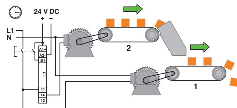
Conveyor belt 2 starts with a time delay
